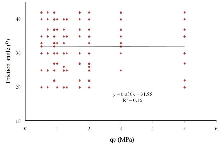
Fig. 12 Correlation between friction with CPT
