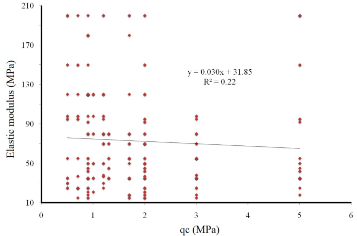
Fig. 14 Correlation between elastic modulus with CPT
