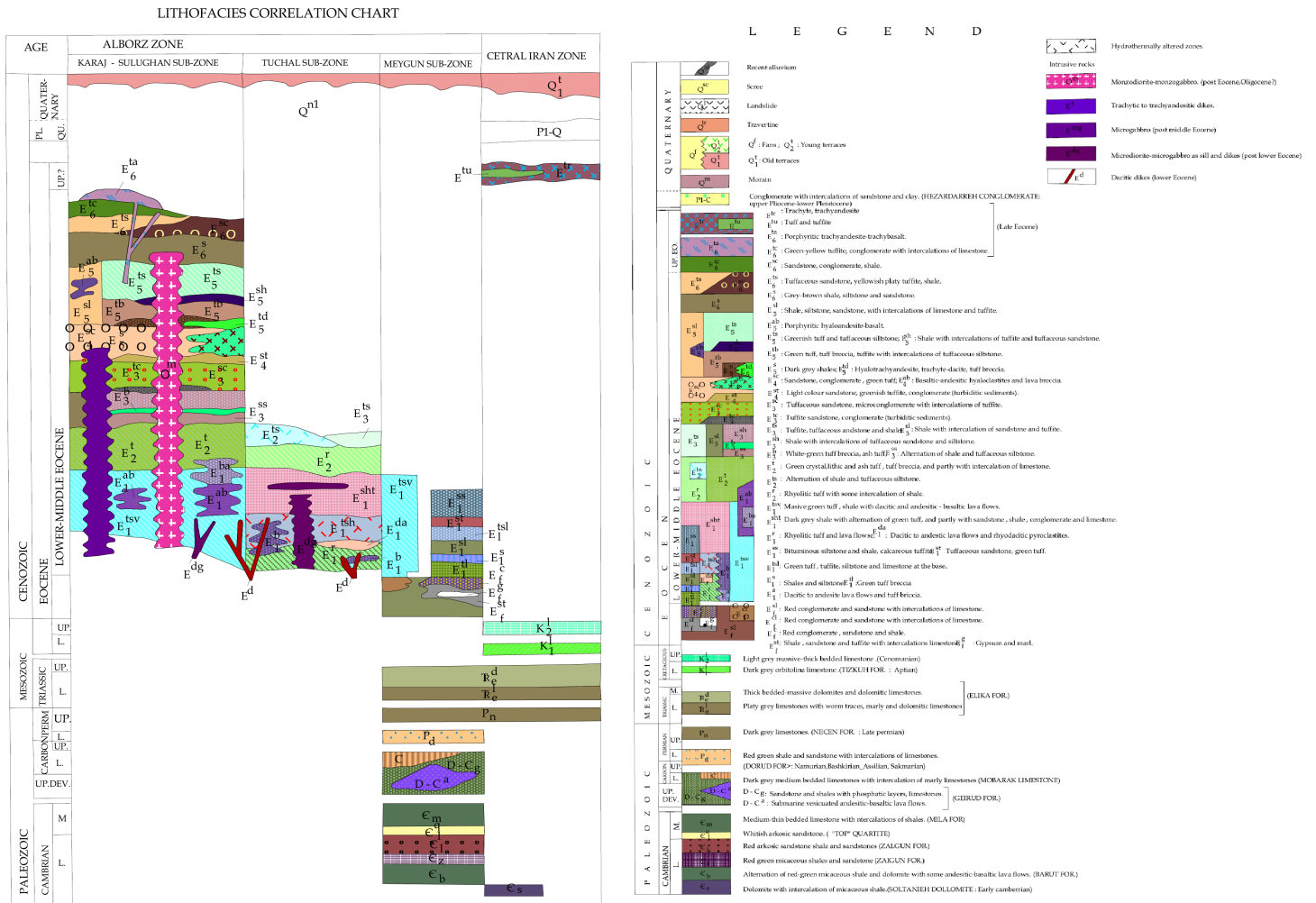
Fig. 3 The stratigraphic chart of Tehran geology (adapted from Geological Survey of Iran, 2010)
