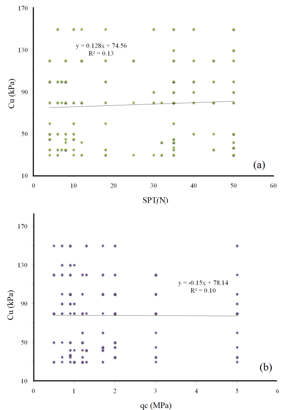
Fig. 15 Correlation between C_u with: (a) SPT, (b) q_c
